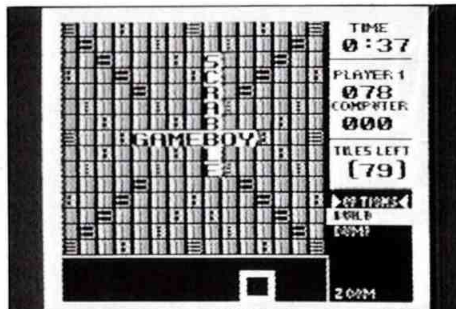
DEMO SCREEN
